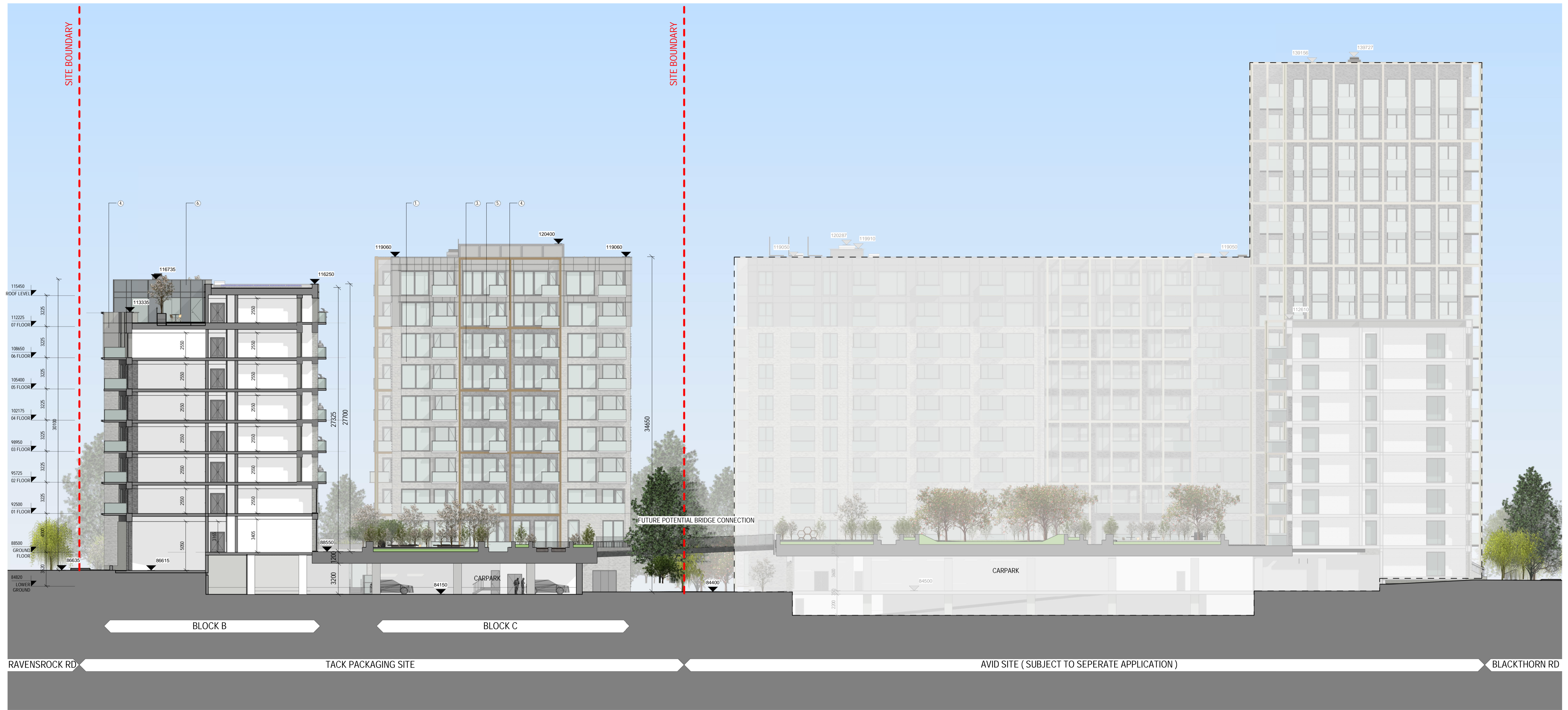
1 SECTION THROUGH PODIUM 01 - TACK SITE 1 : 200
